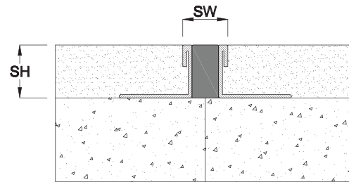
Straight Application YCS (Stainless Steel)
